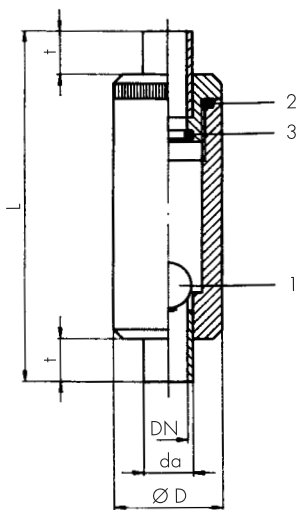
Filler and breather valve V91
