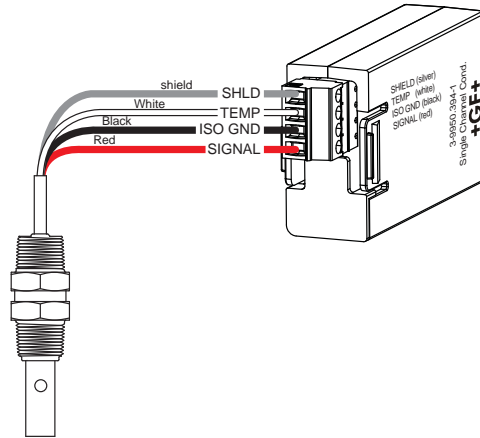
Single channel Conductivity Module
