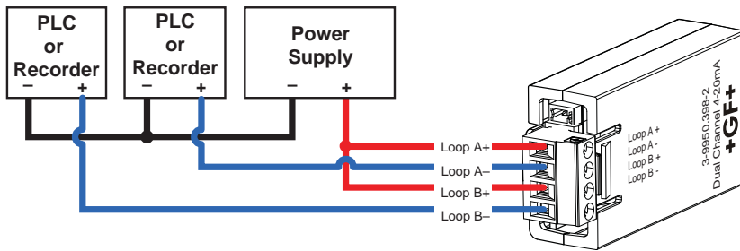
Dual Channel 4 to 20 mA Module
